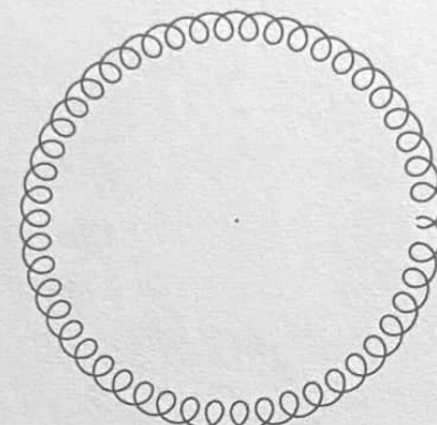
MERCURY - JUPITER
