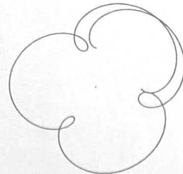
MERCURY - EARTH
