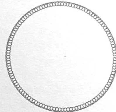
MERCURY - SATURN
