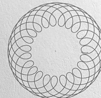
SATURN - NEPTUNE
