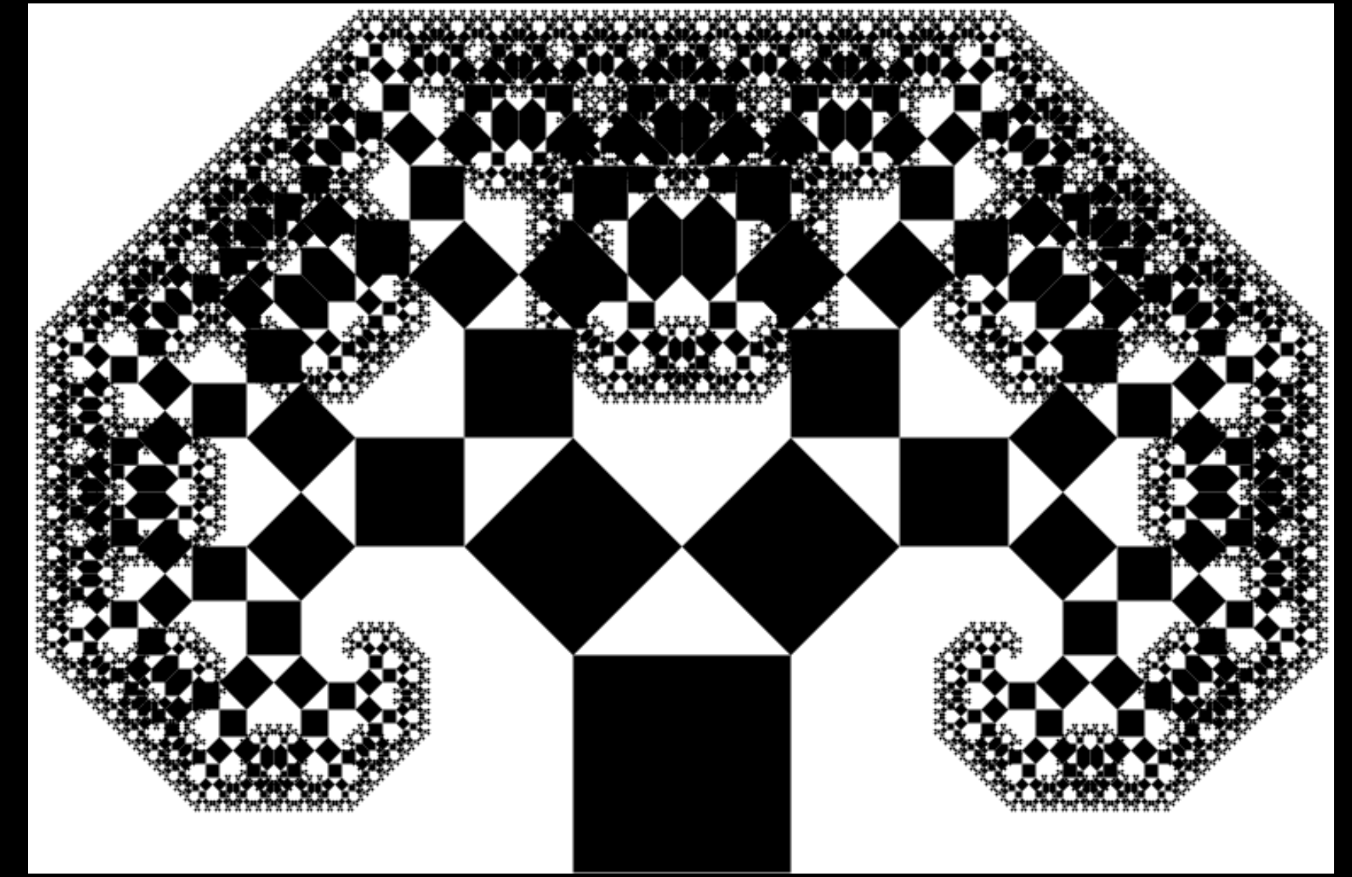
Pythagoras Tree
