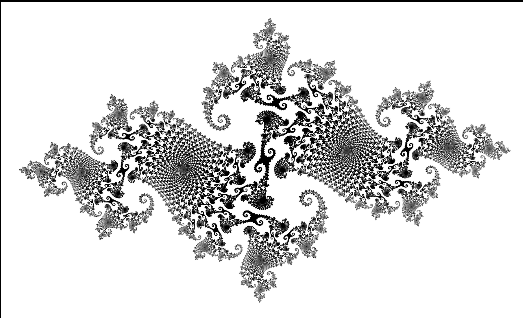
Julia Set
