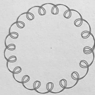
MERCURY - CERES
