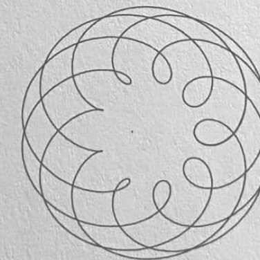
CHIRON - NEPTUNE
