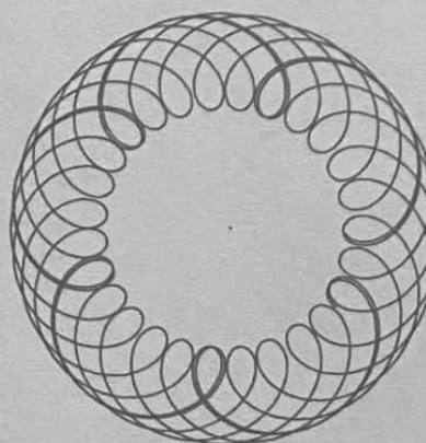
CERES - SATURN
